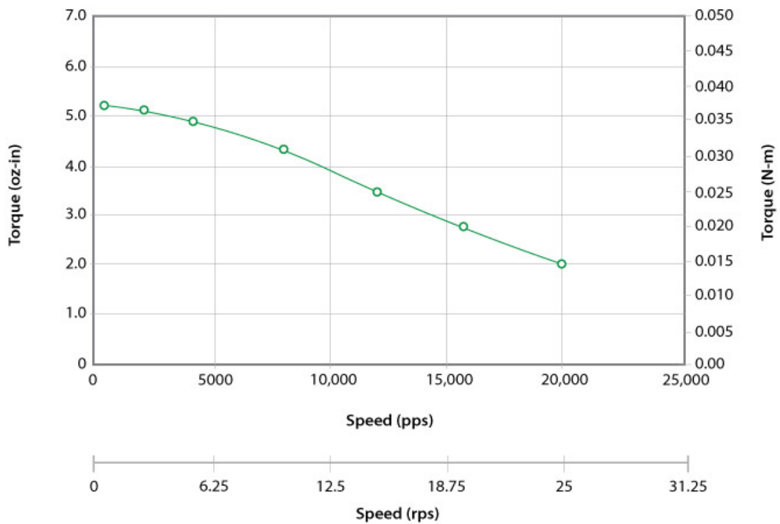
3809X-15 24VDC, 0.3 Amps/Phase, Bipolar, 1/2 Stepping
